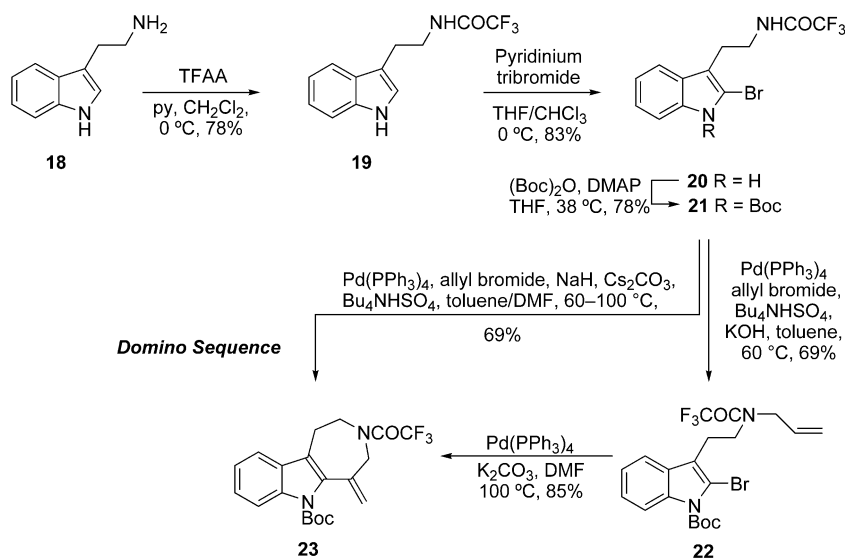
Scheme 4. Construction of the azepino[4,5- b ]indole ring system through single-step or domino Tsuji–Trost/Heck reactions.
