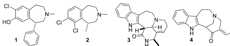
Figure 1. Structures of interesting 3-benzazepines and azepino[4,5- b ]indoles natural products.
