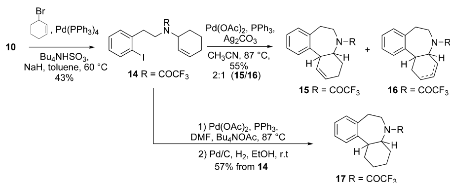
Scheme 3. Construction of the octahydrodibenzazepine ring system through single-step Tsuji–Trost and Heck reactions.
