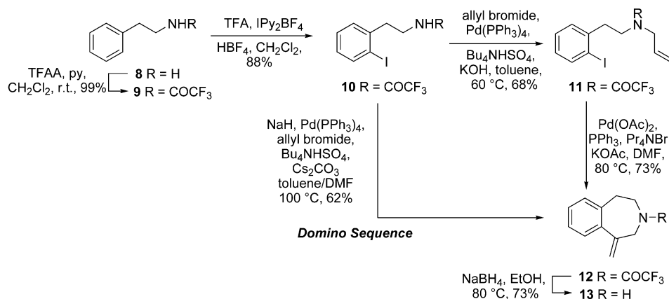
Scheme 2. Construction of the 3-benzazepine ring system through single-step or domino Tsuji-Trost/Heck reaction.
