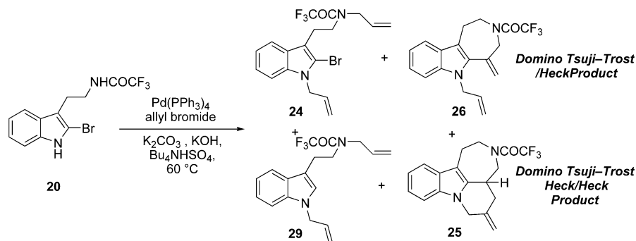
Scheme 6. Domino Tsuji–Trost/Heck cross-coupling to produce tricycle 26 and accompanying domino Tsuji–Trost/Heck/Heck reaction to produce tetracycle 25 .
