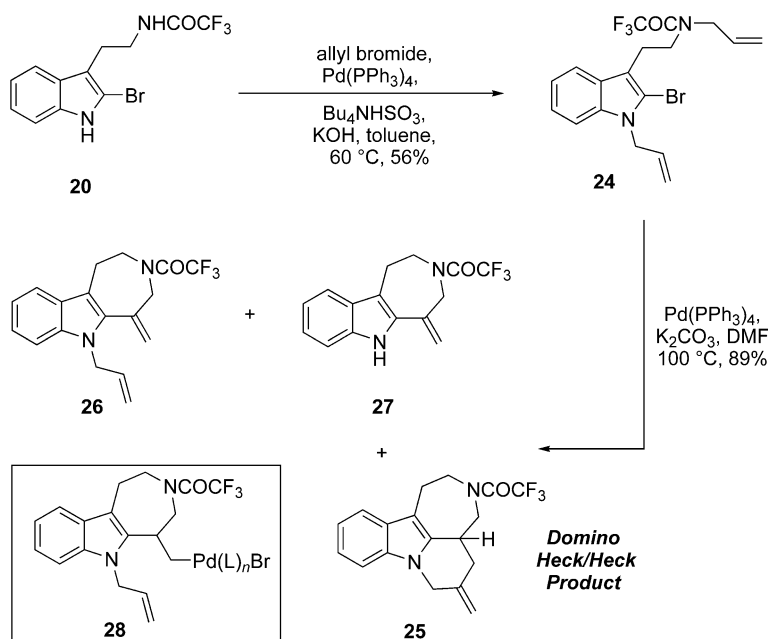
Scheme 5. Synthesis of allylazepino[4,5- b ]indoles and azepinobenzindolizine ring systems through a Heck and domino Heck/Heck reaction.
