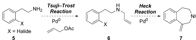
Scheme 1. Proposed domino Tsuji-Trost/Heck reaction.
